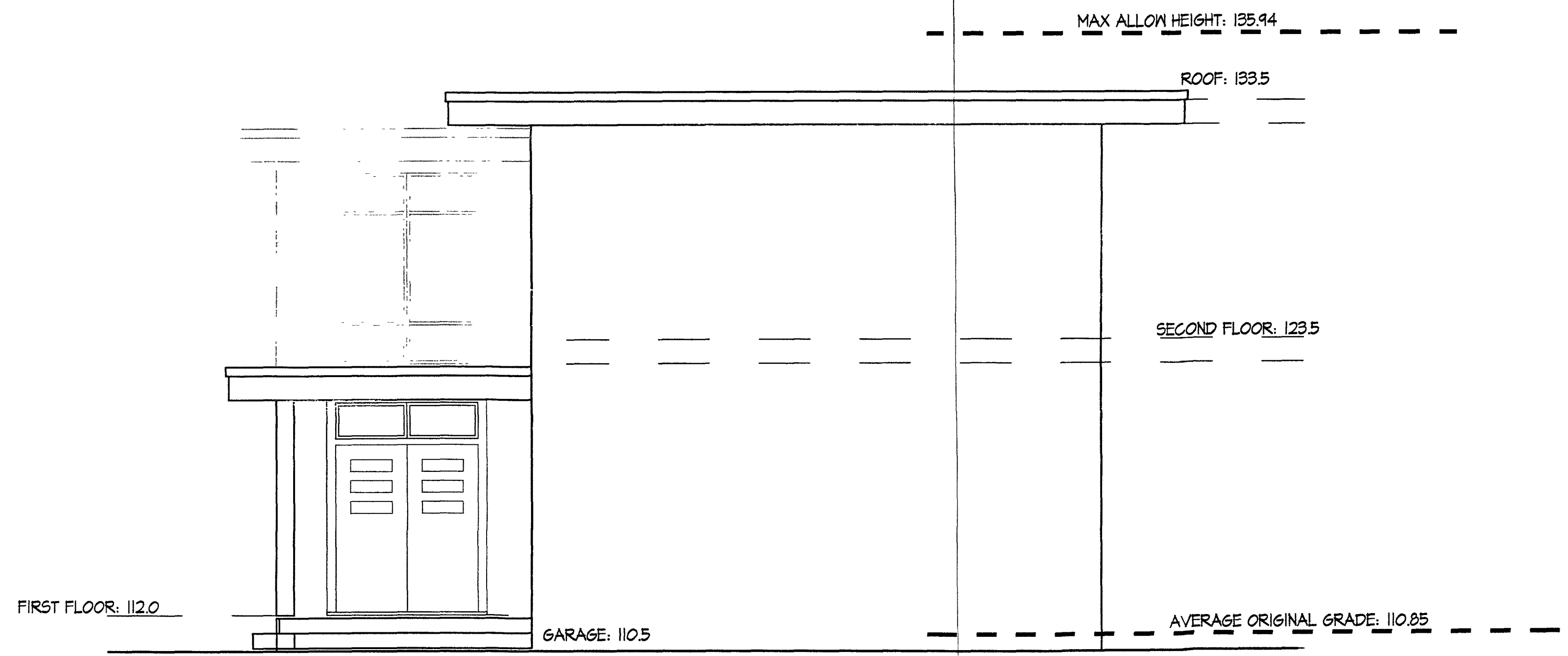
EAST ELEVATION
